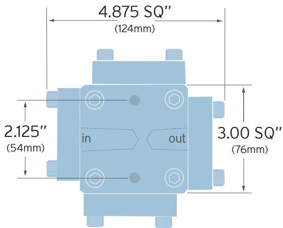
MODEL 214 WITH INDUSTRIAL HOUSING TRANSMITTER
